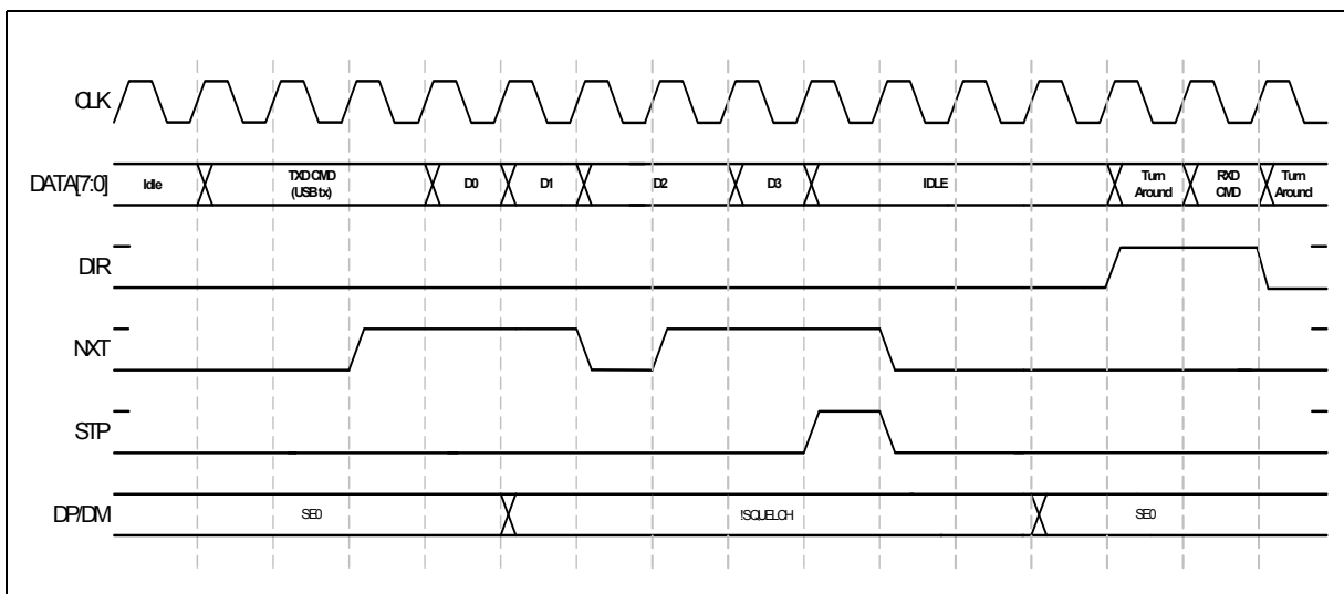
FIGURE 6-6: ULPI TRANSMIT
