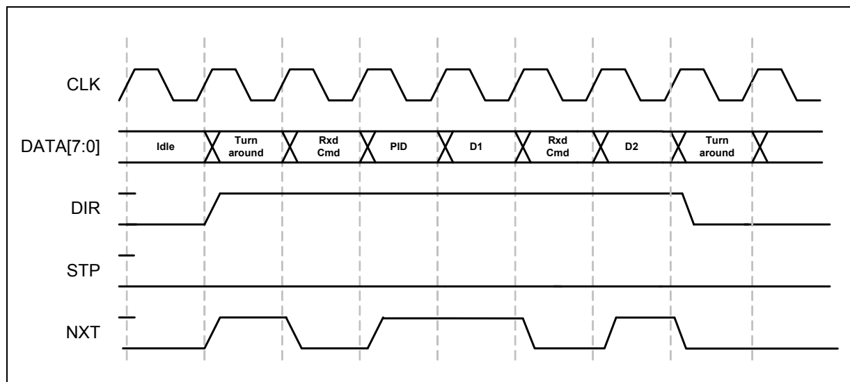
FIGURE 6-7: ULPI RECEIVE
