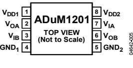
Figure 5. ADuM1201 Pin Configuration
