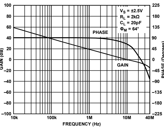
Figure 15. Open-Loop Gain and Phase vs. Frequency
