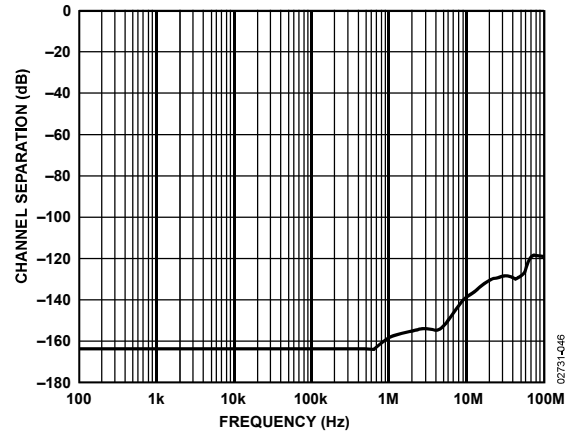
Figure 49. Channel Separation vs. Frequency
