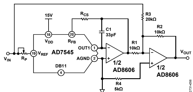
Figure 59. Bipolar Operation
