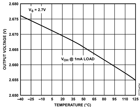
Figure 35. Output Voltage Swing High vs. Temperature
