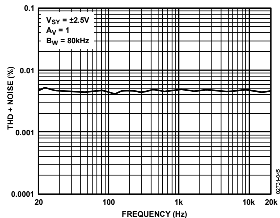
Figure 48. THD + Noise vs. Frequency
