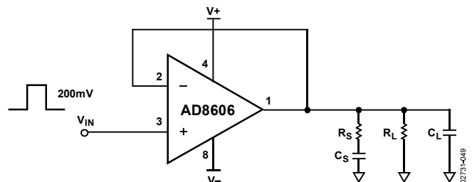
Figure 51. Snubber Network Configuration
