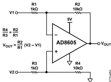
Figure 56. Difference Amplifier, A_V = 10
