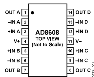
Figure 4. 14-Lead SOIC_N (R Suffix)
