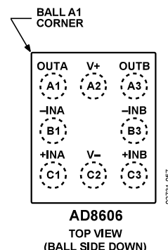
Figure 2. 8-Ball WLCSP (CB Suffix)
