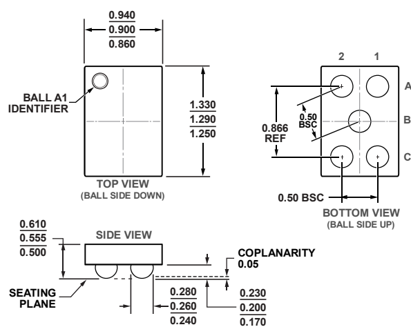
Figure 60. 5-Ball Wafer Level Chip Scale Package [WLCSP] (CB-5-1)
