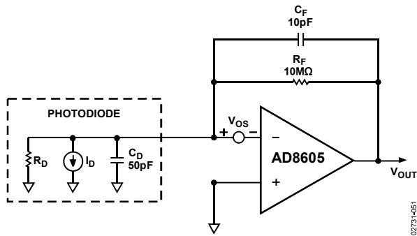
Figure 54. Equivalent Circuit for Photodiode Preamplifier
