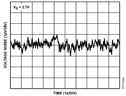
Figure 41. 0.1 Hz to 10 Hz Input Voltage Noise
