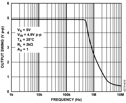
Figure 16. Closed-Loop Output Voltage Swing (FPBW)
