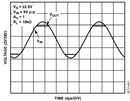
Figure 46. No Phase Reversal
