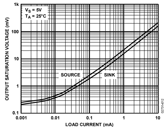
Figure 12. Output Saturation Voltage vs. Load Current
