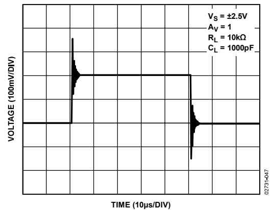
Figure 50. AD8606 Capacitive Load Drive Without Snubber
