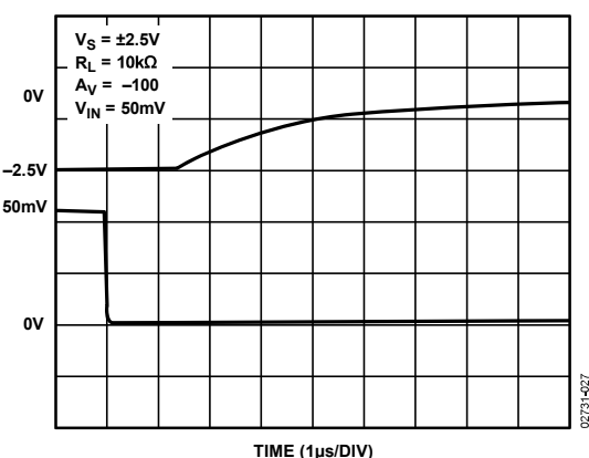
Figure 27. Negative Overload Recovery
